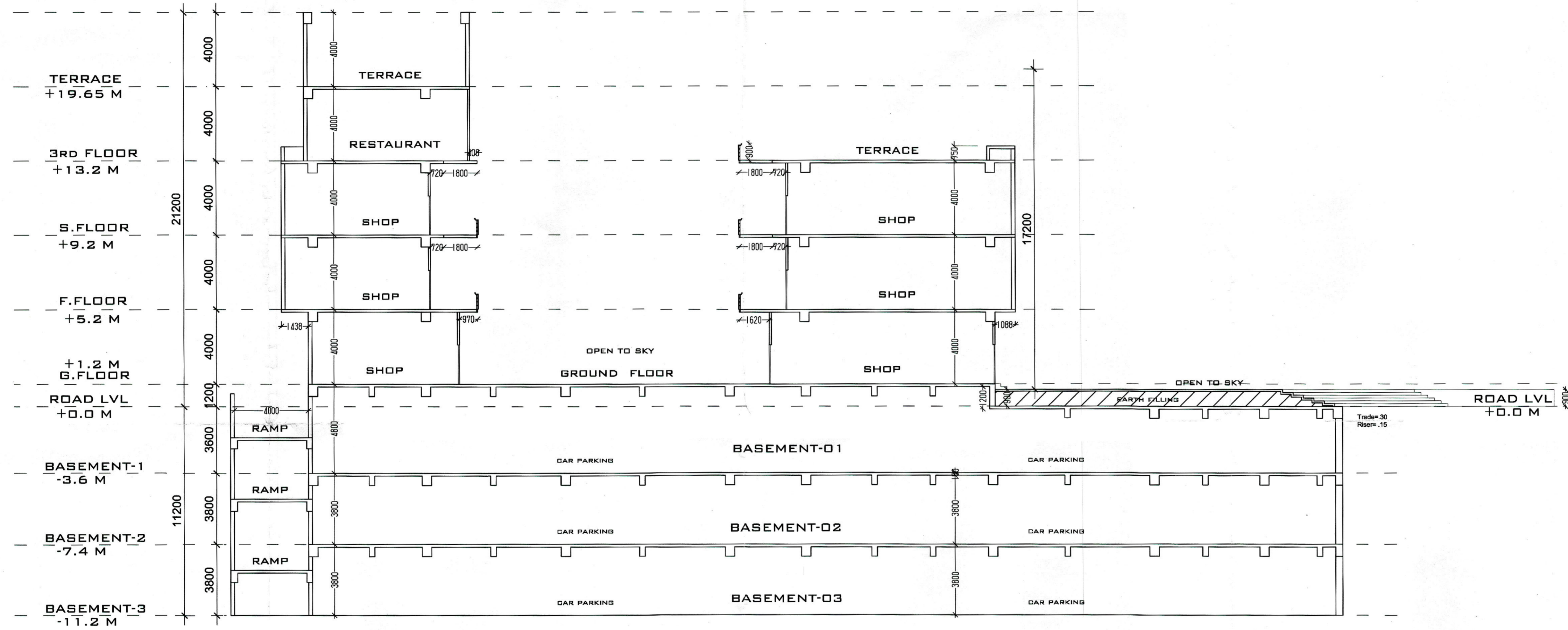
SECTION- C-C
